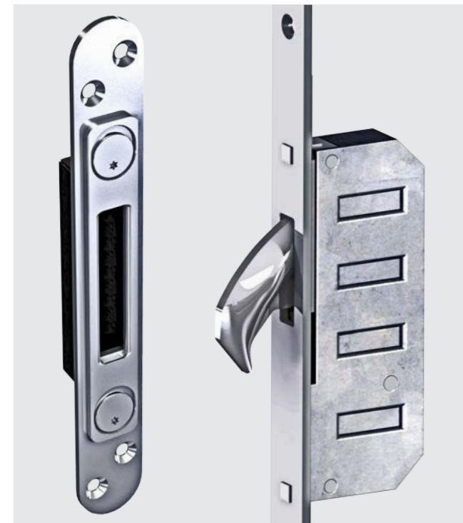
Standard 24mm wide keeps with dust boxes and off-set screw fixing for enhanced security.
